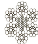
6 x 19S (9/9/1)
