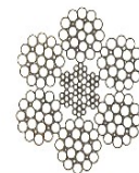
6 x 25FW (12/6 & 6F/1)
